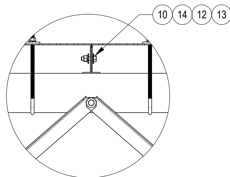
DETAIL A SCALE 5 : 28
