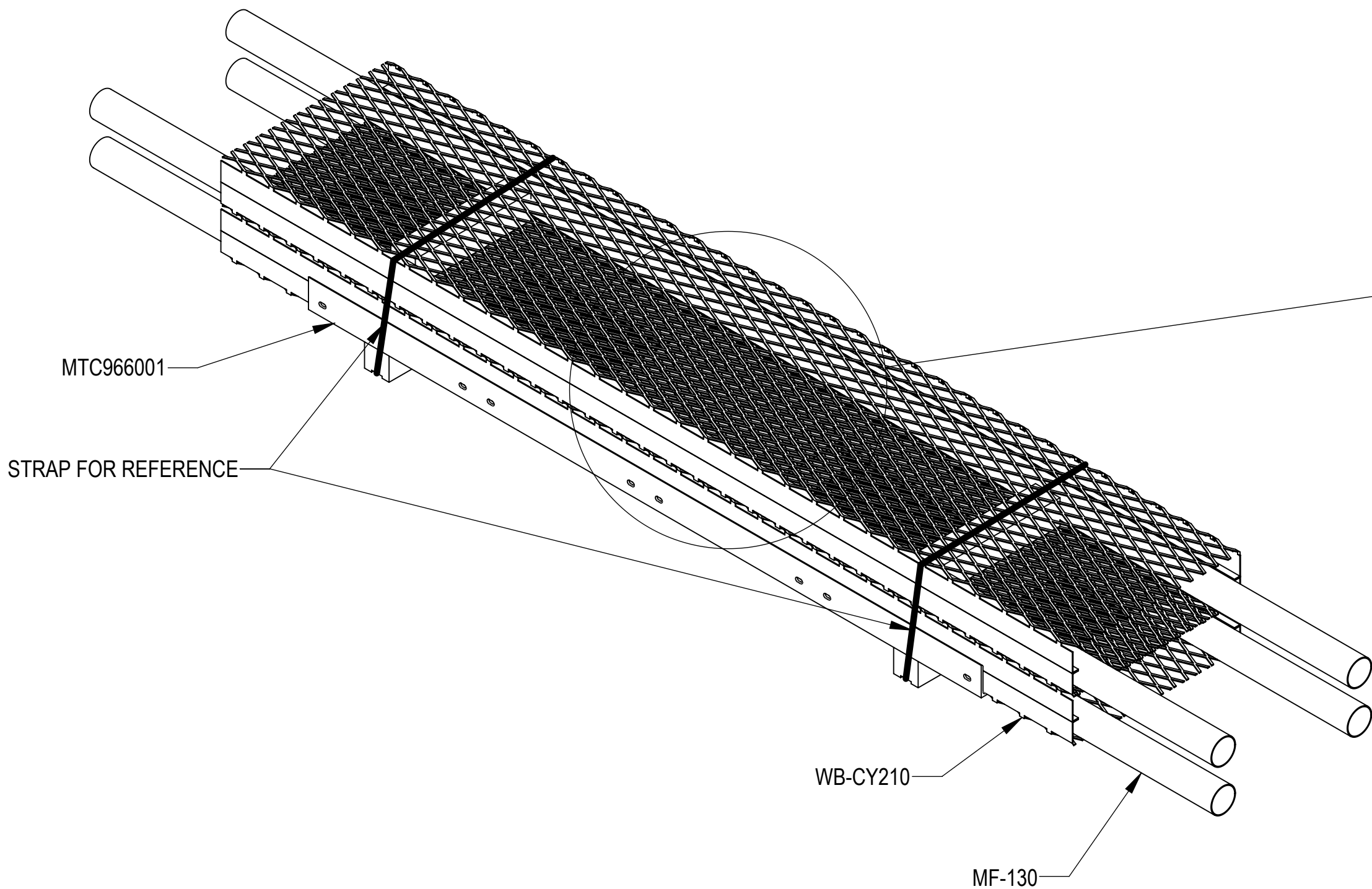
PACKAGE VIEW
