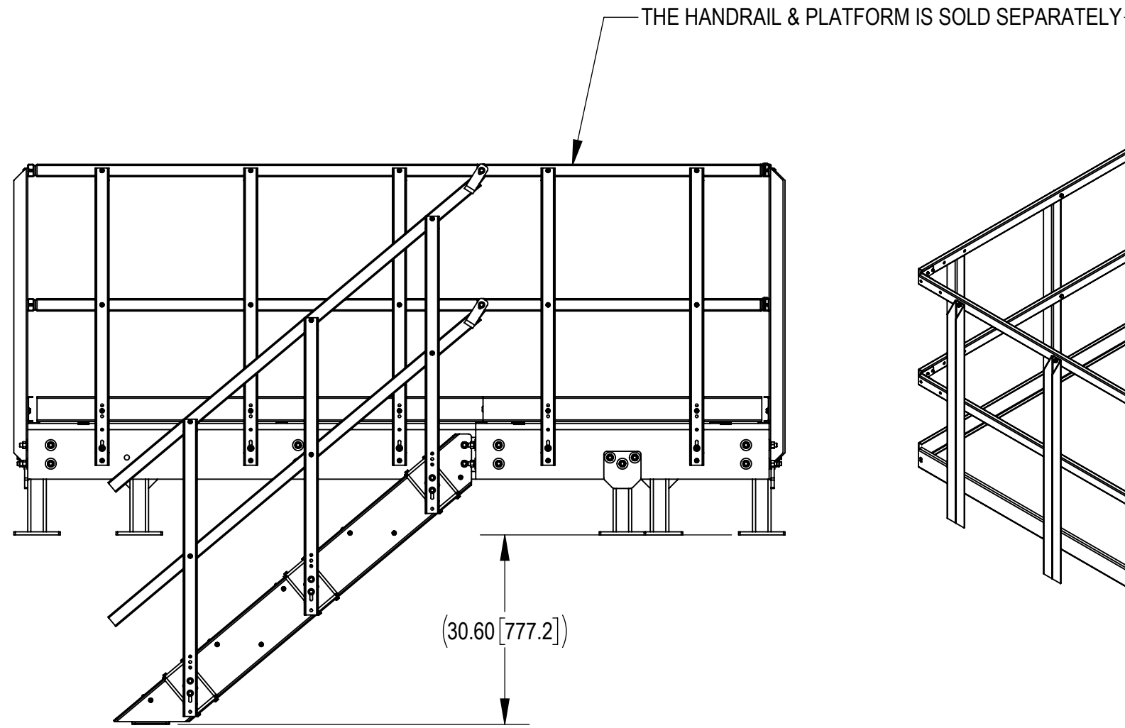
STAIR WITH EQP0404L-DSH & EQP0404LHR-DSH PLATFORM (SOME PARTS OF PLATFORM ARE HIDDEN FOR CLARITY)
