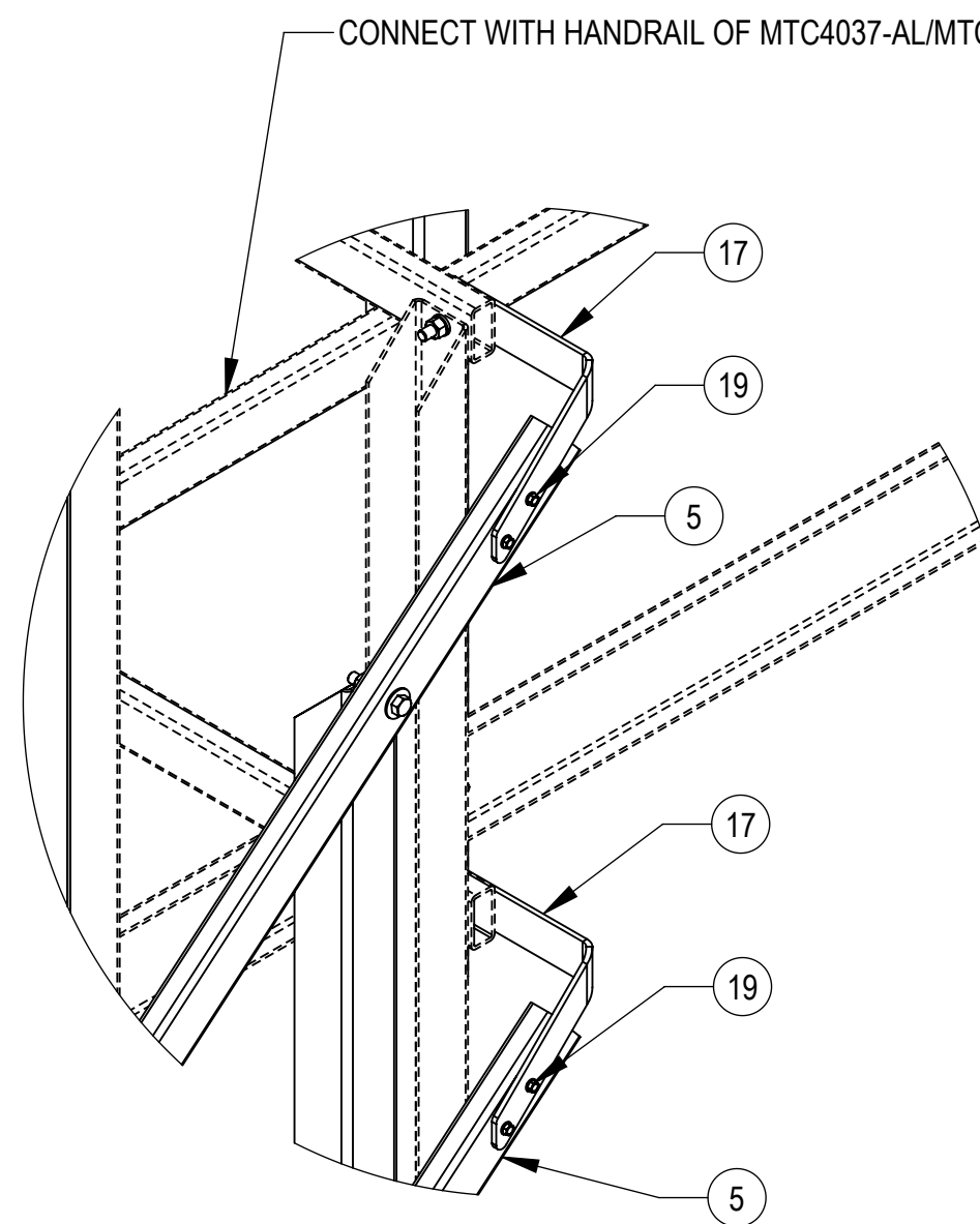
DETAIL E SCALE 1 : 6
