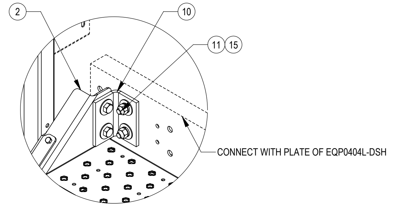
DETAIL R SCALE 1 : 6
