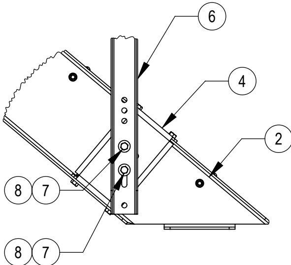
SECTION S-S SCALE 1 : 8
