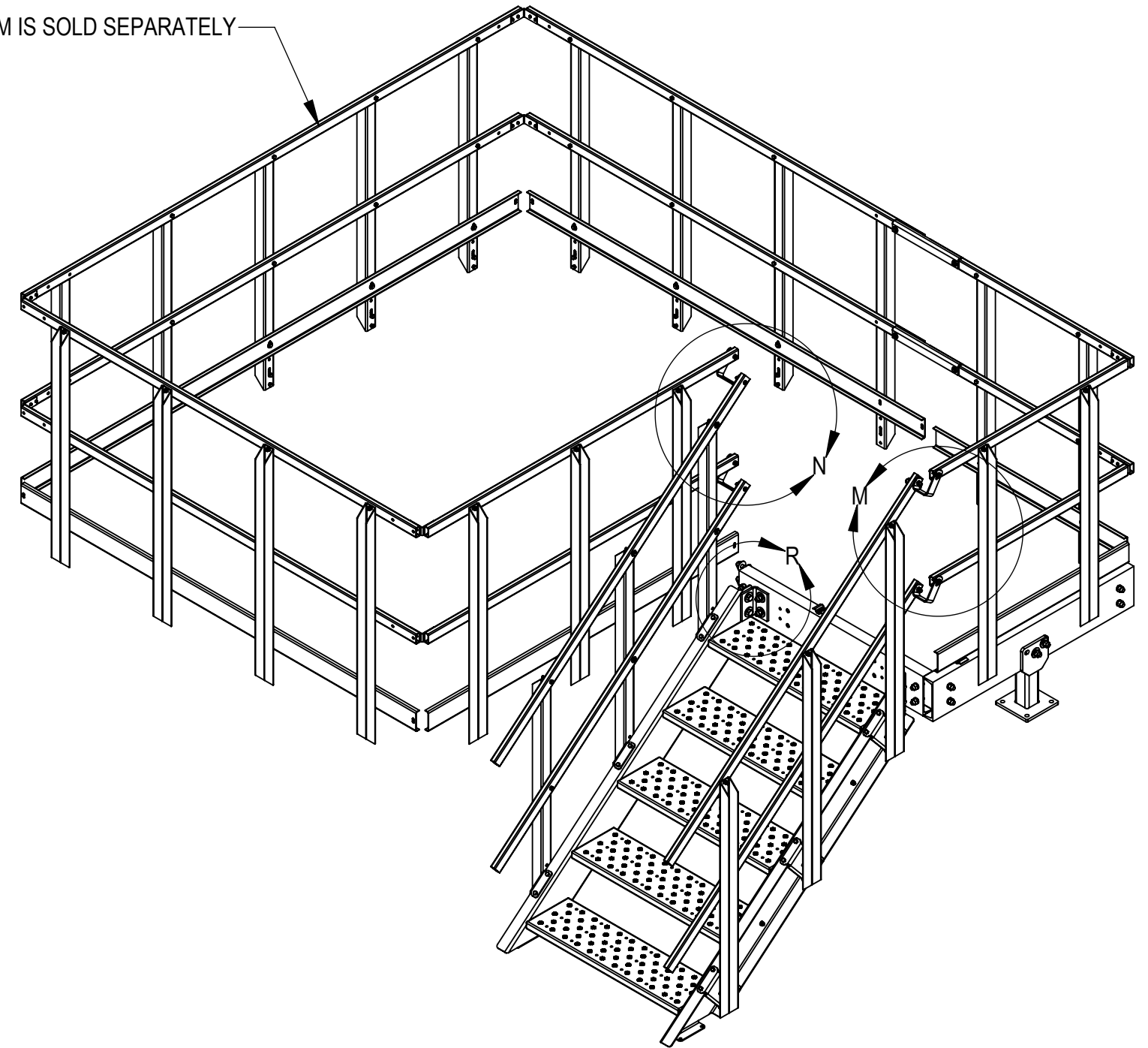
STAIR WITH EQP0404L-DSH & EQP0404LHR-DSH PLATFORM (SOME PARTS OF PLATFORM ARE HIDDEN FOR CLARITY)
