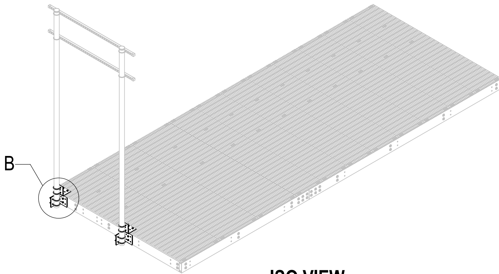
ISO VIEW
