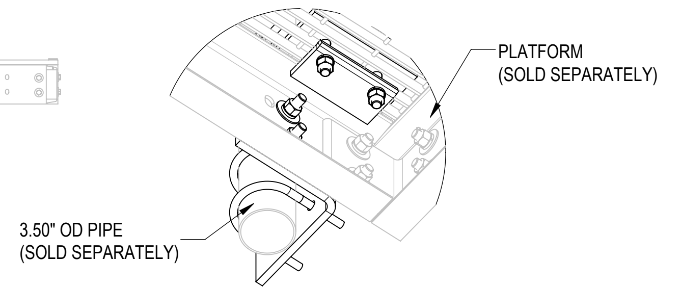
OPPOSITE VIEW FOR DETAIL B SCALE 1 : 6
