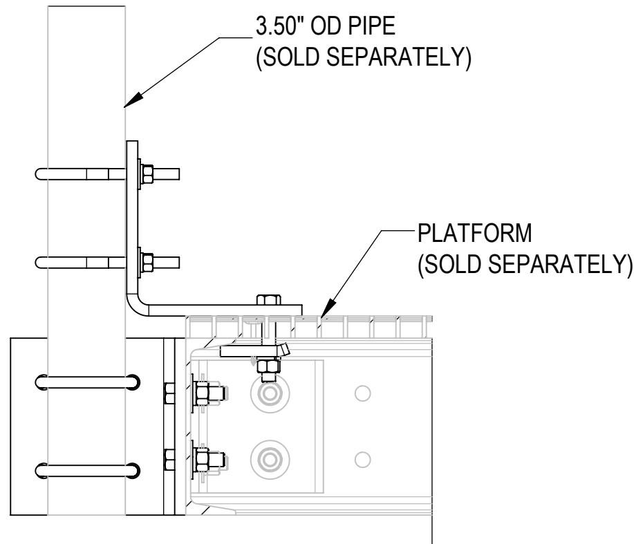
SECTION A-A CROP VIEW SCALE 1 : 6
