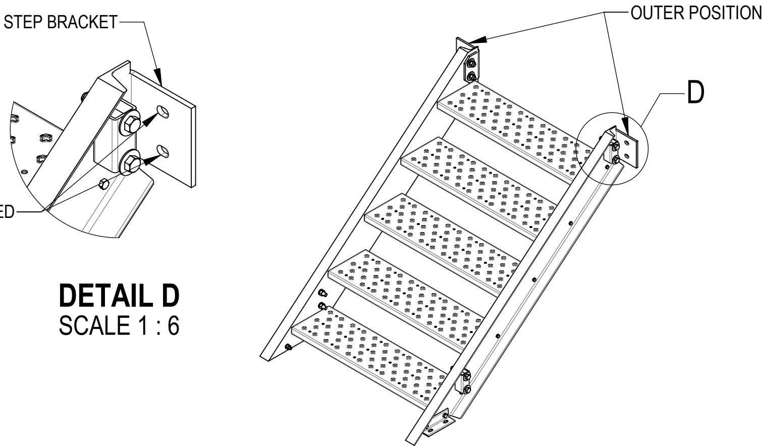
OUTWARD BRACKET ORIENTATION
