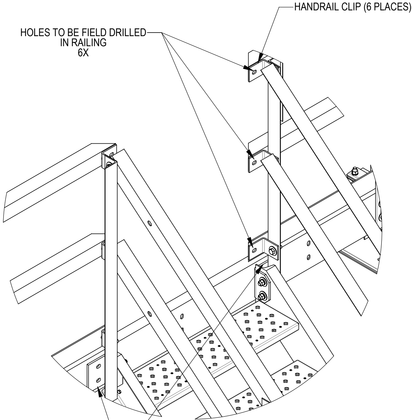
DETAIL F SCALE 1 : 10
