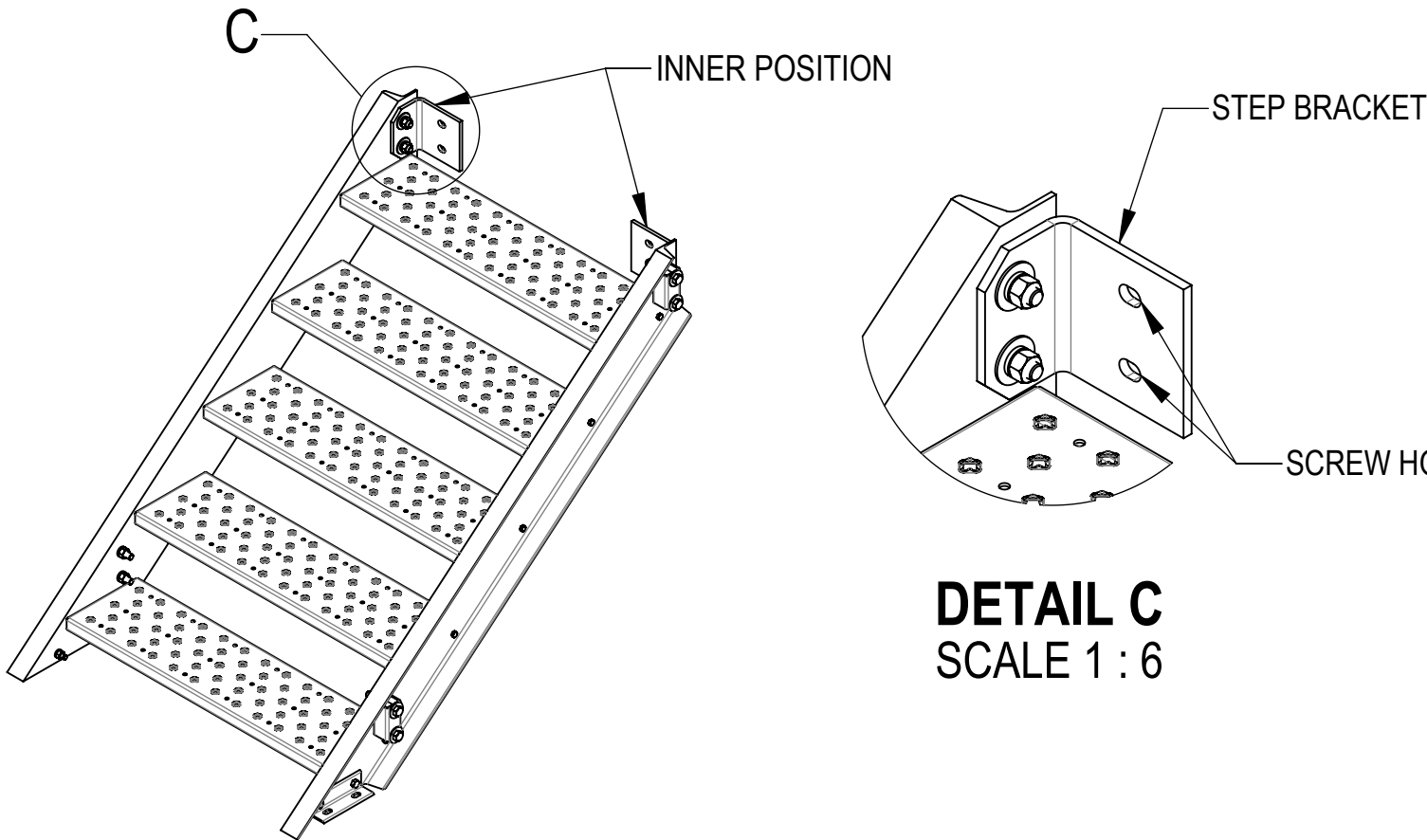
INWARD BRACKET ORIENTATION
