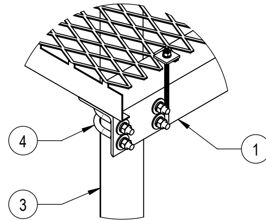
DETAIL A SCALE 1 : 8
