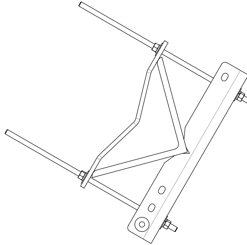
90 ° TOWER LEGS UP TO 12" X 12" ANGLE
