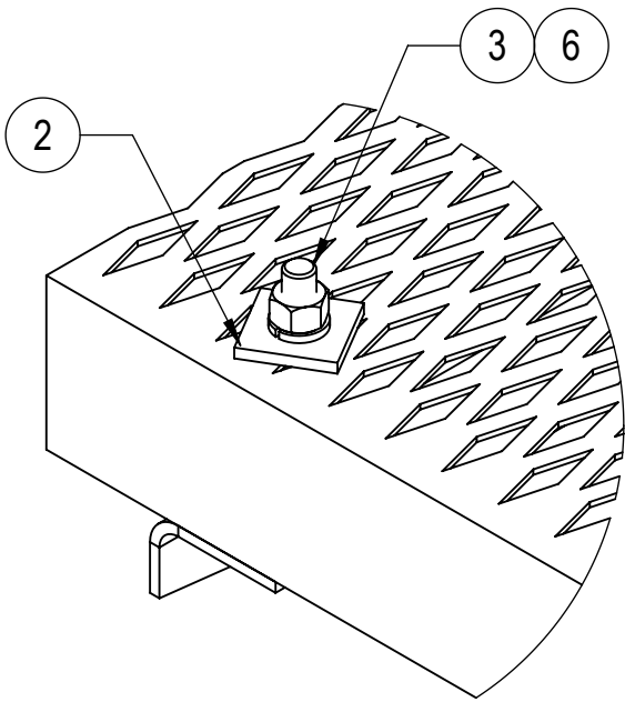
DETAIL A SCALE 1 : 3
