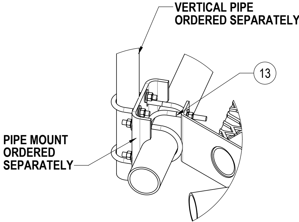
DETAIL E SCALE 1 : 6
