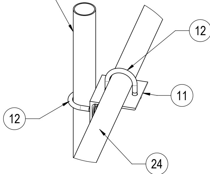
DETAIL D SCALE 1 : 6
