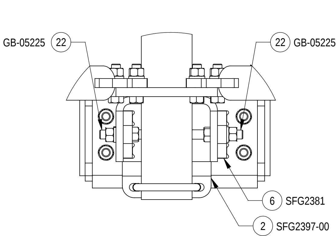
DETAIL FRONT VIEW OF BOTTOM MOUNT SCALE 1 : 4
