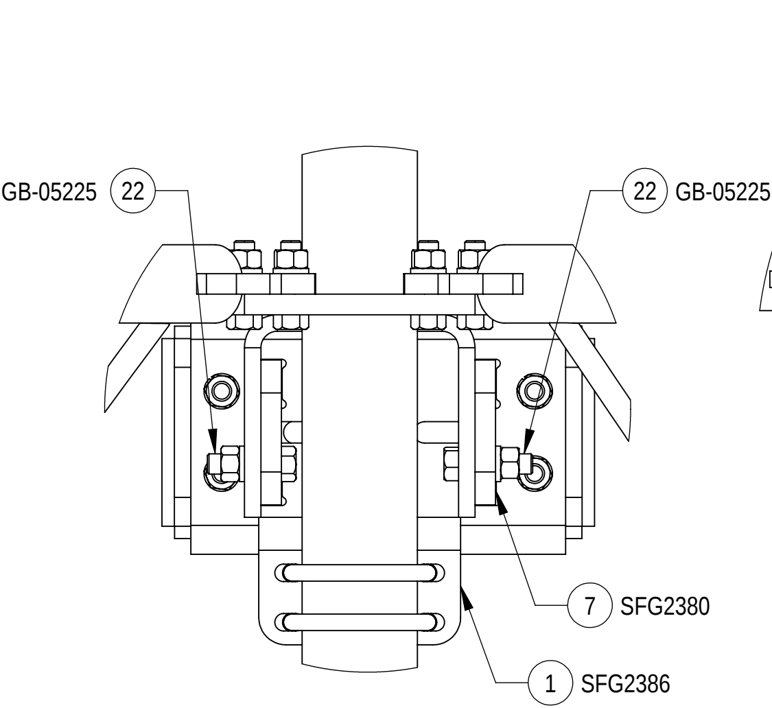
DETAIL FRONT VIEW OF TOP MOUNT SCALE 1 : 4
