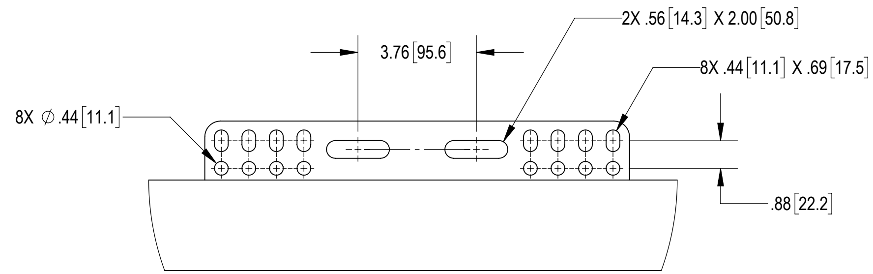
DETAIL P SCALE 1 : 3
