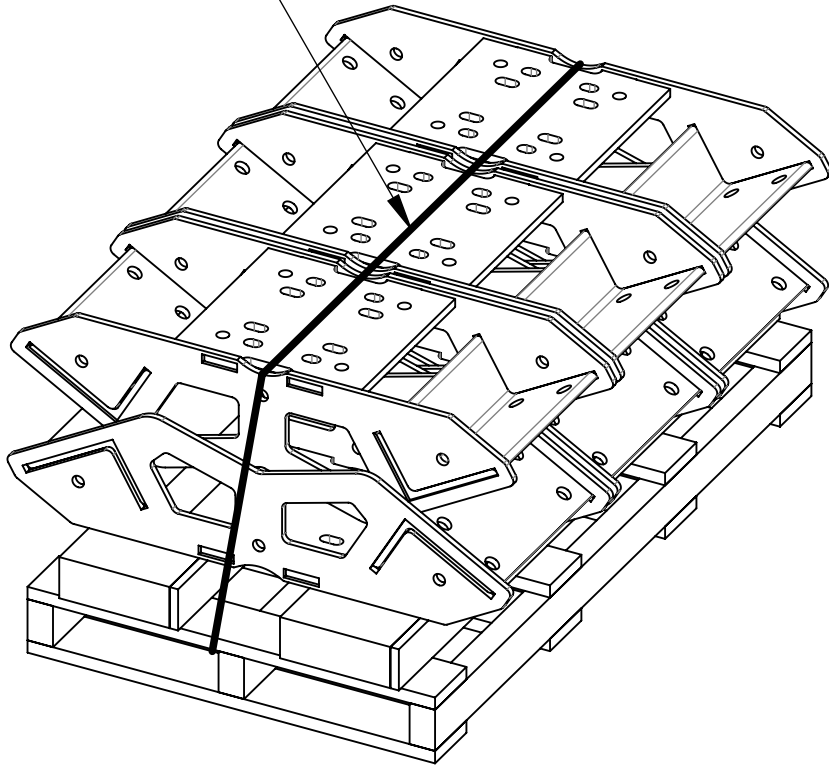
RING MOUNT
