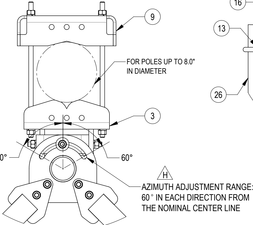
DETAIL C SCALE 1 : 6
