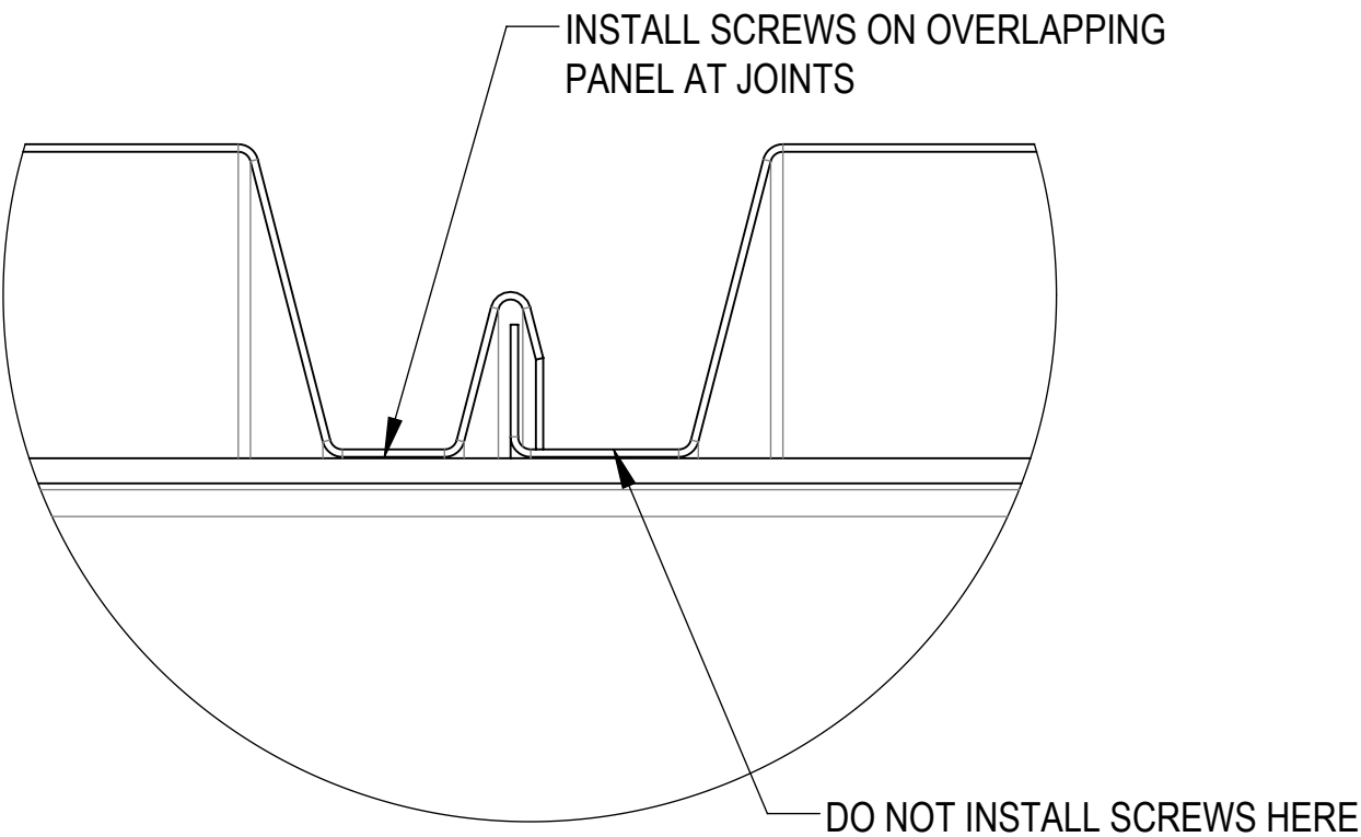
DETAIL B SCALE 1 : 1
