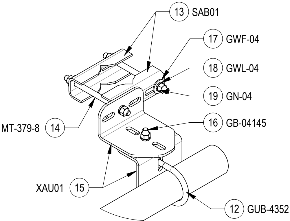
DETAIL R SCALE 1 : 5
