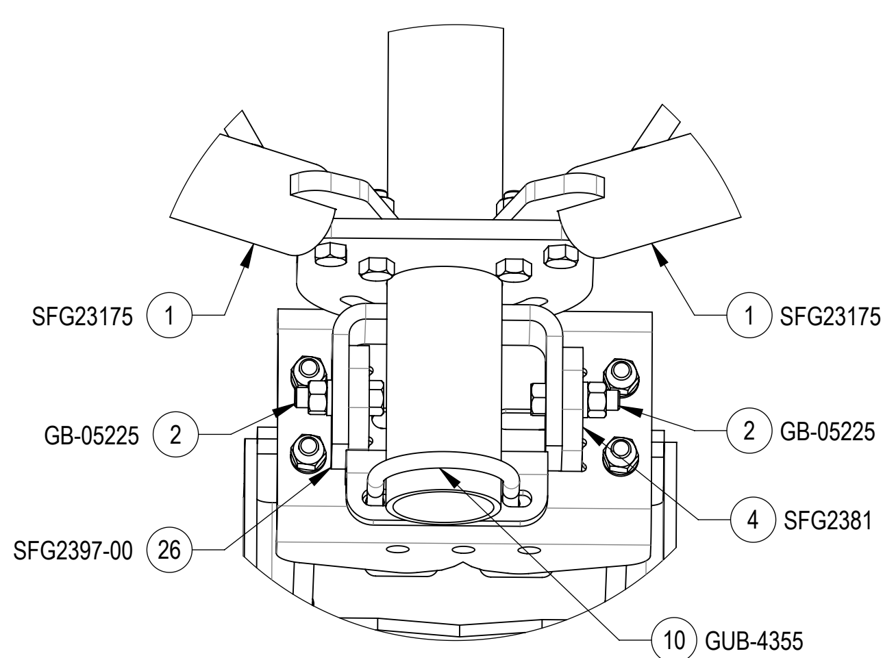
DETAIL ISO BOTTOM ROTATED VIEW SCALE 1 : 4
