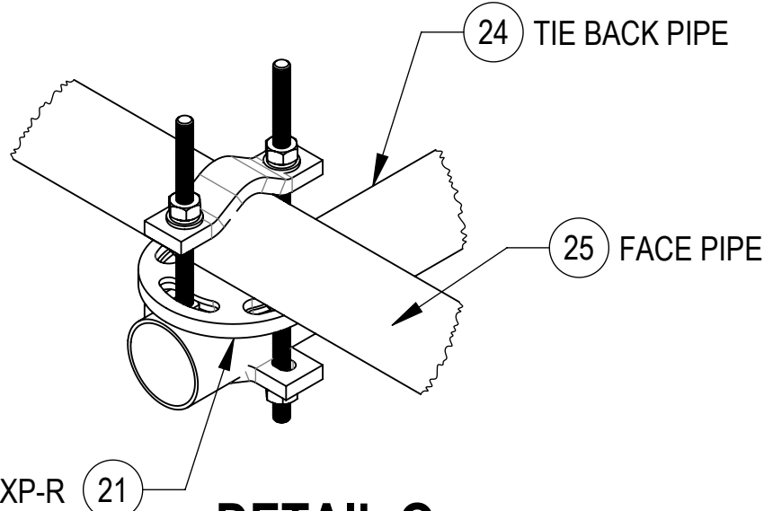
DETAIL Q SCALE 1 : 5
