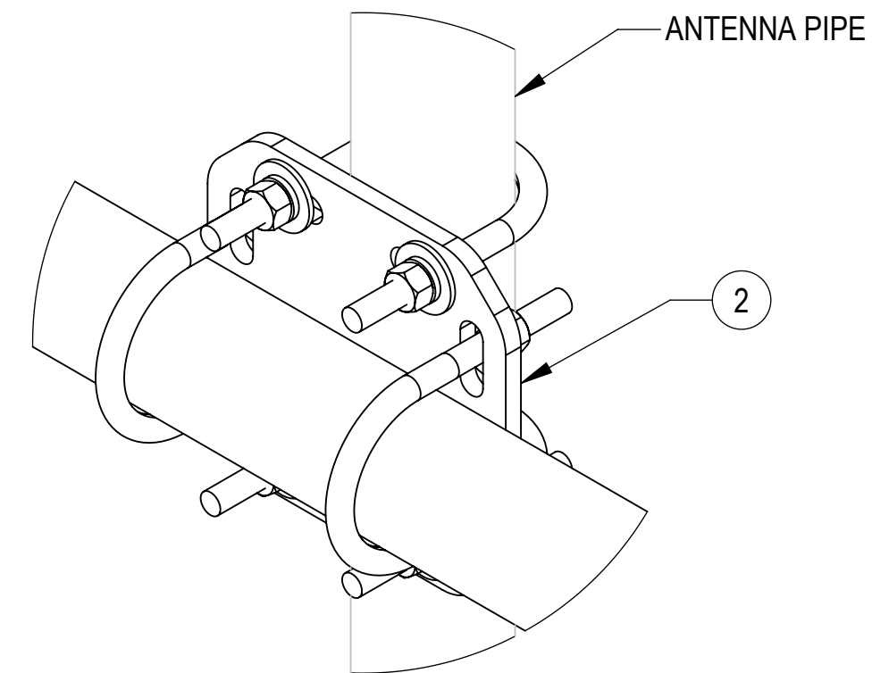
DETAIL B SCALE 1 : 3
