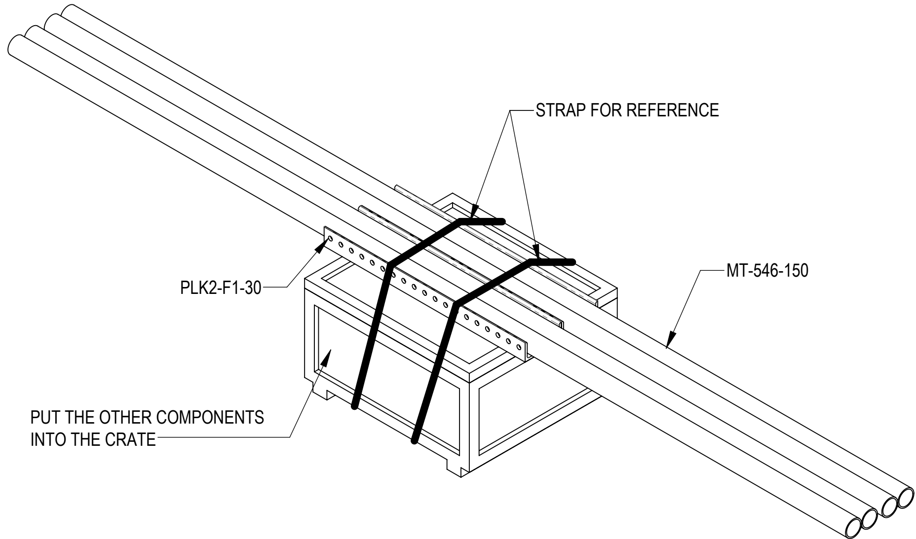
PACKAGE VIEW
