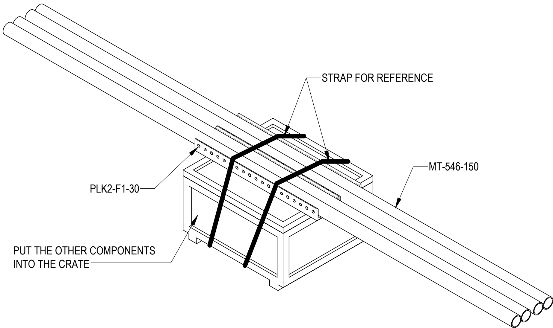
PACKAGE VIEW
