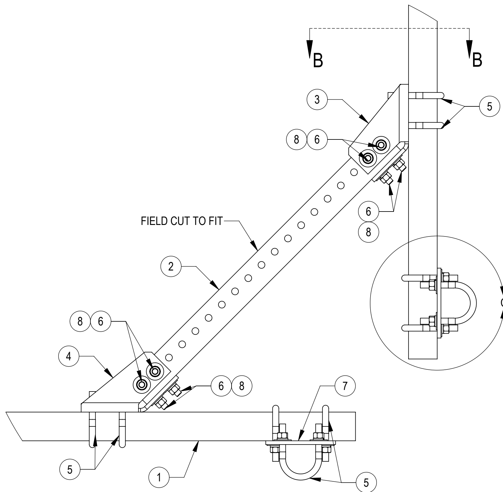
DETAIL A SCALE 1 : 6
