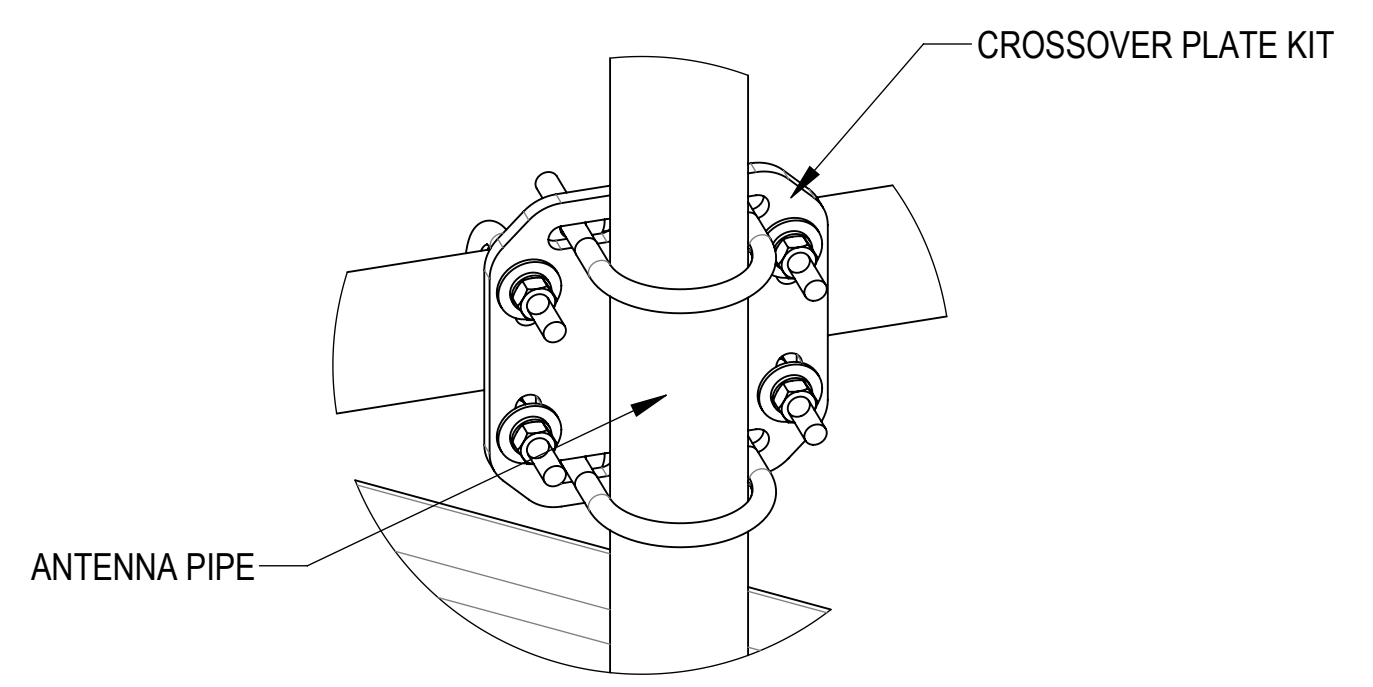
DETAIL C SCALE 1 : 4
