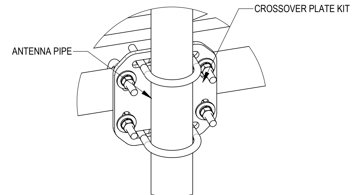
DETAIL C SCALE 1 : 4
