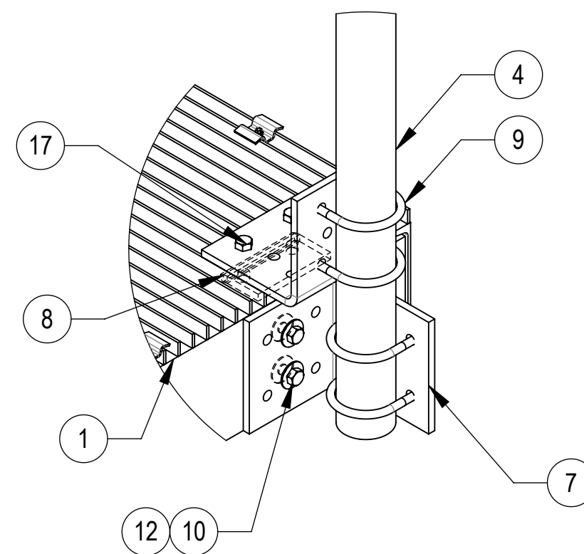
DETAIL B SCALE 1 : 8
