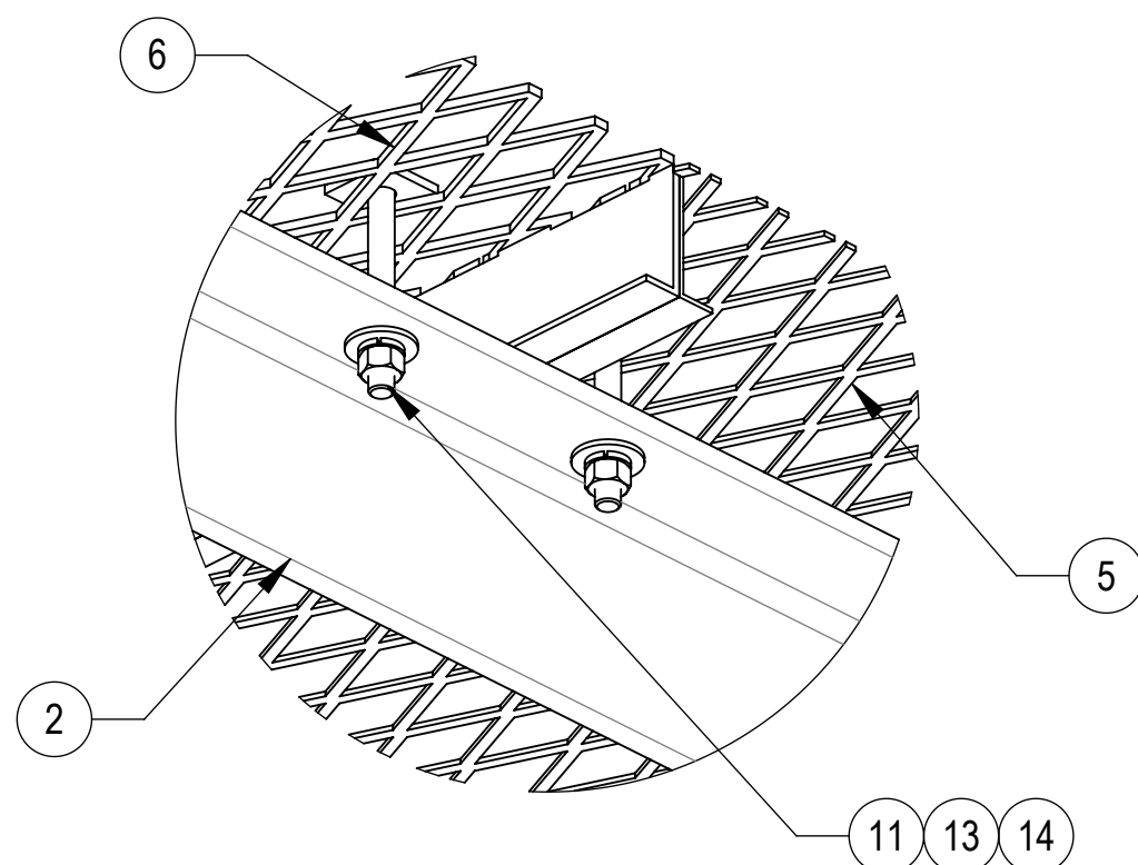
DETAIL E SCALE 1 : 4
