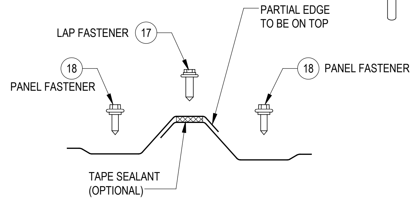
TYPICAL PANEL JOINT DETAIL
