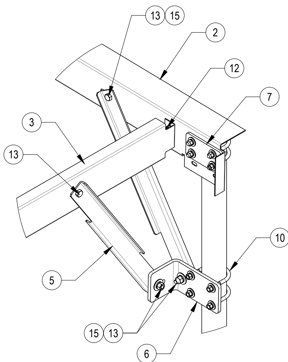
DETAIL B SCALE 1 : 8
