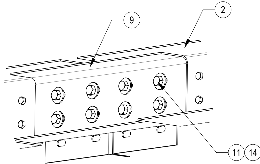
DETAIL E BACK VIEW SCALE 1 : 4
