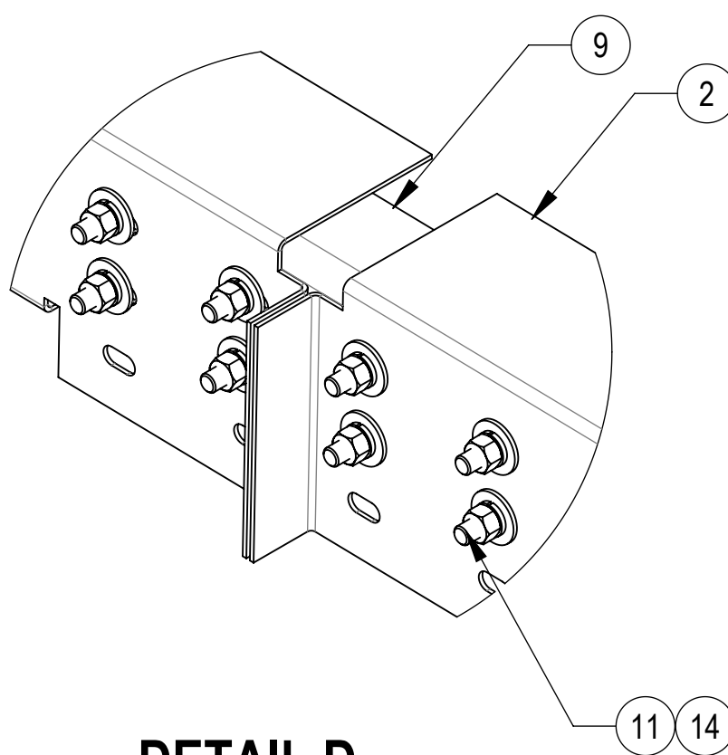
DETAIL D SCALE 1 : 4
