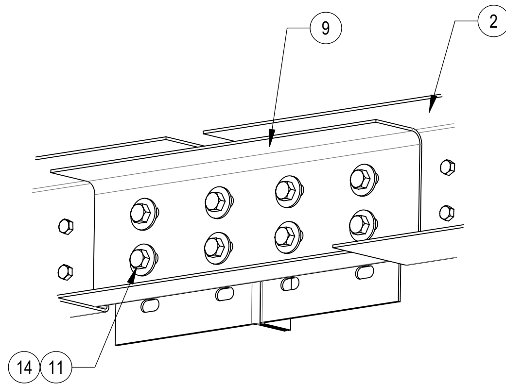
DETAIL D BACK VIEW SCALE 1 : 4
