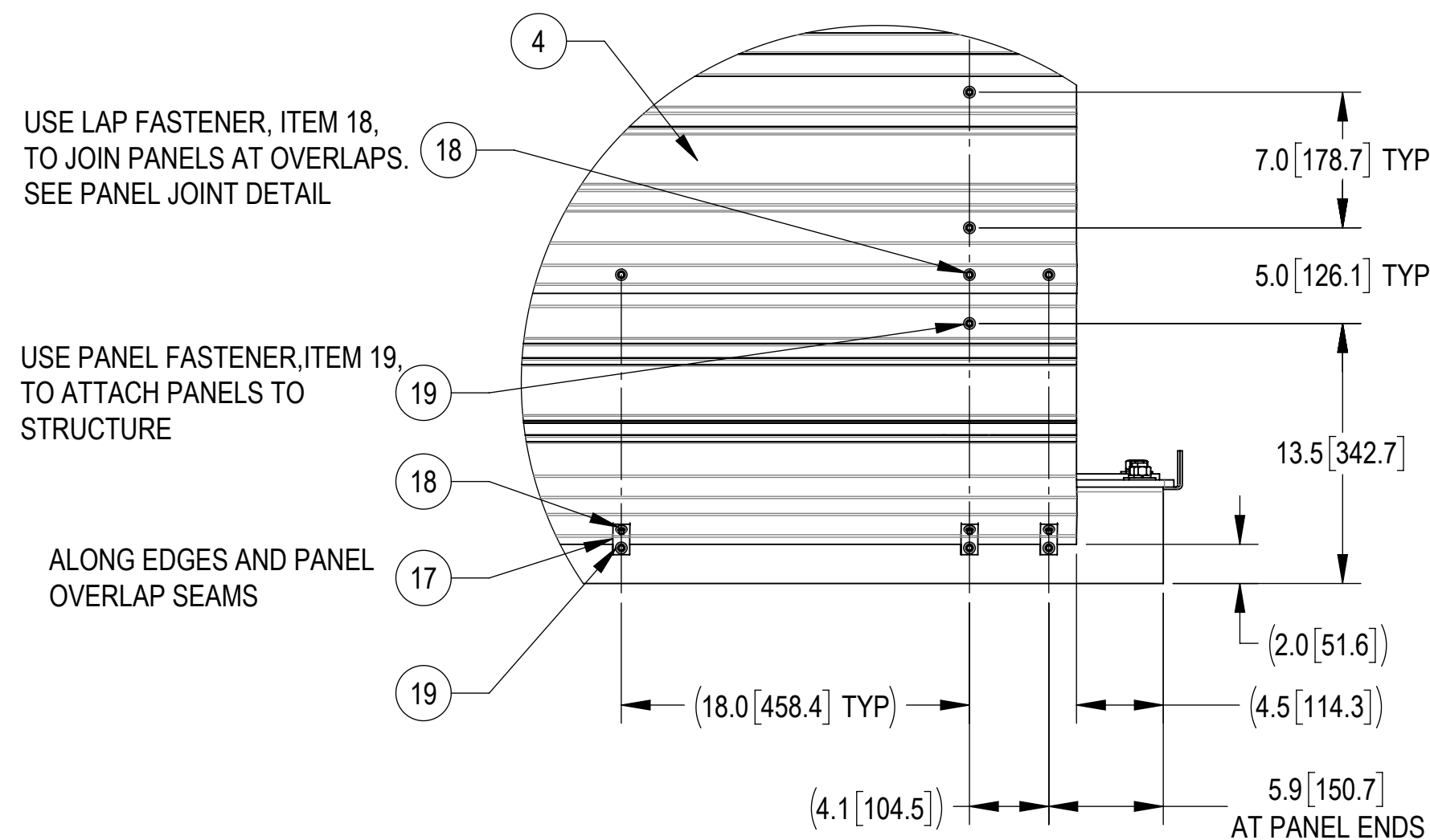
DETAIL E SCALE 1 : 8
