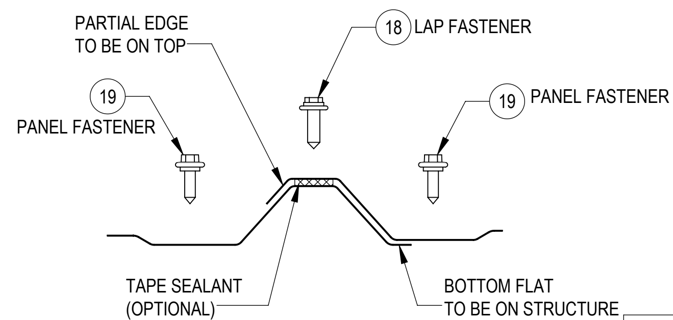
TYPICAL PANEL JOINT DETAIL
