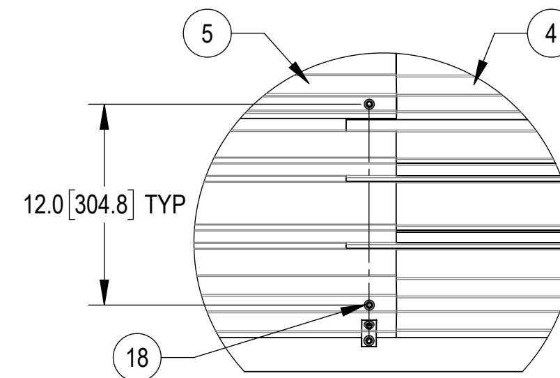
DETAIL F SCALE 1 : 8
